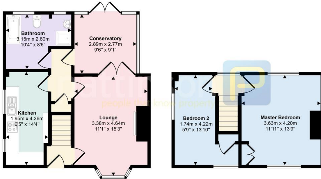
First Floor Approx 28 sq m / 305 sq ft
